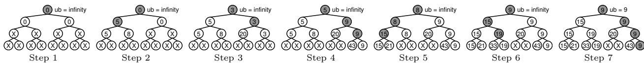
Figure 5: Execution Trace of ADOPT with the Maximum Amount of Memory
