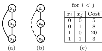
Figure 1: Example DCOP Problem
