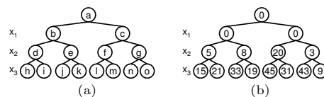
Figure 2: Search Tree
