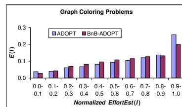
Figure 7: Correlation of \hat{E}(I) and E(I)
